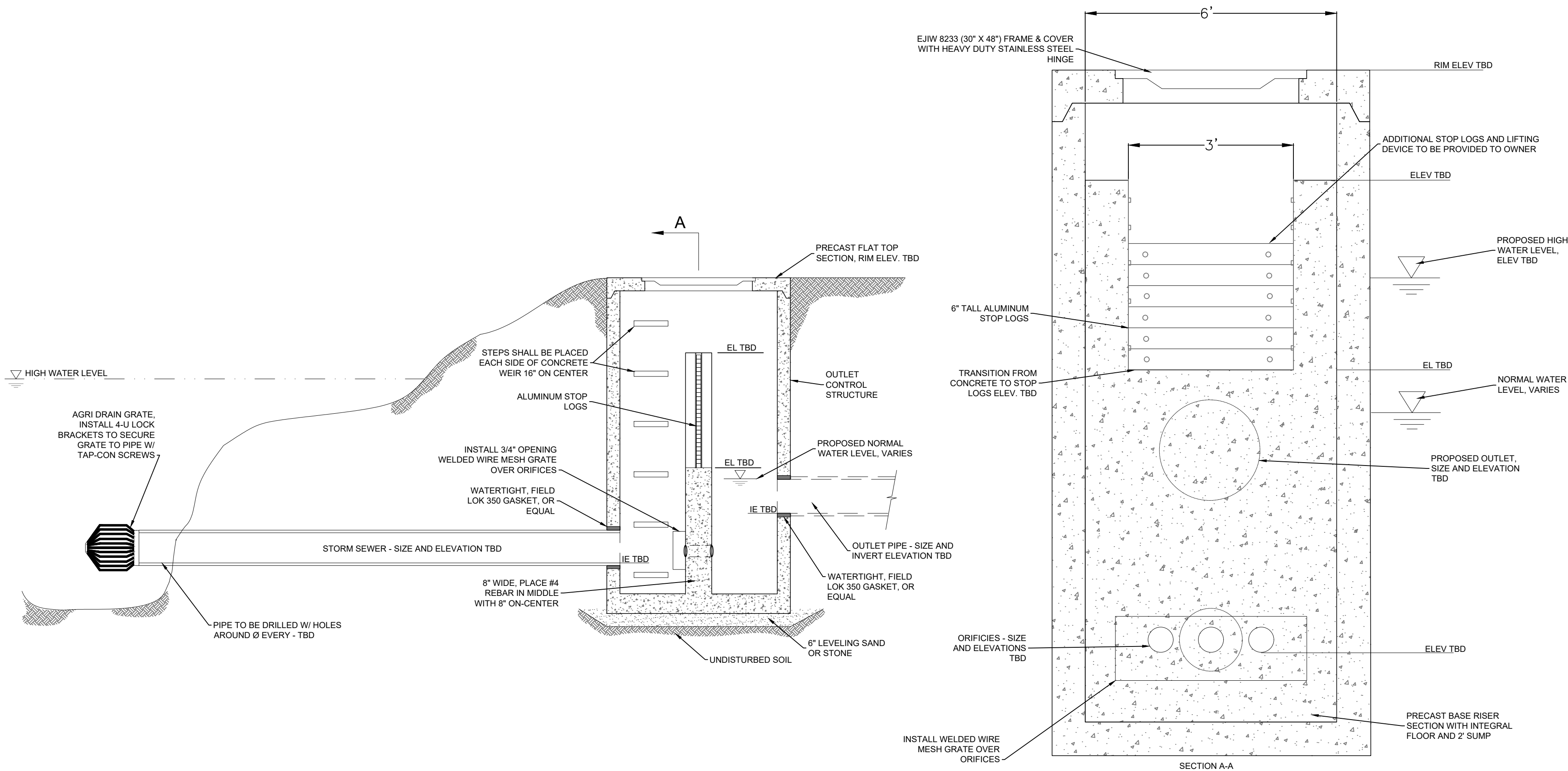
TYPICAL LAKE CONTROL STRUCTURE NO SCALE
